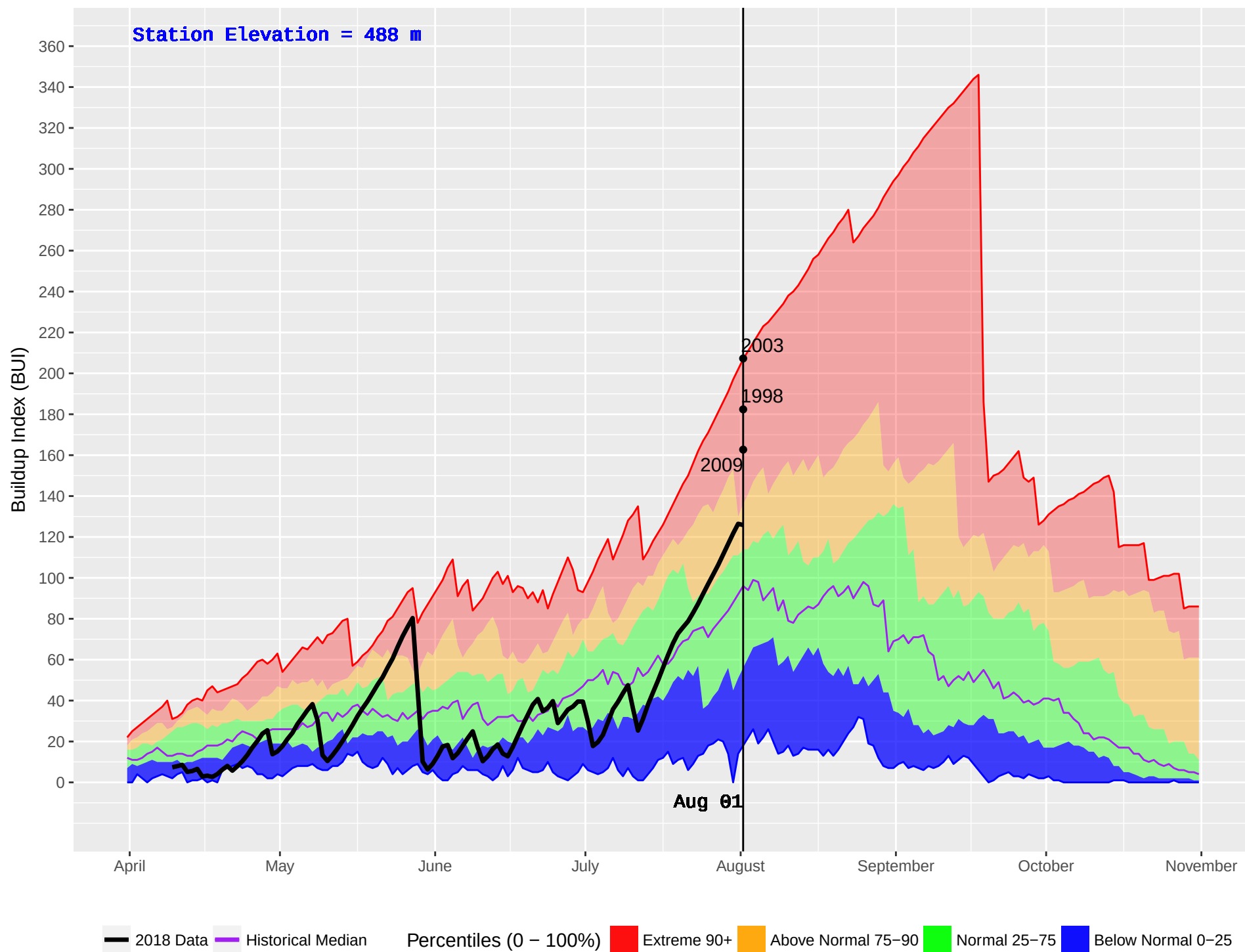
MABEL LAKE 2 (362) : Historical (1987–2016) and Current (2018) Daily Buildup Index (BUI)
