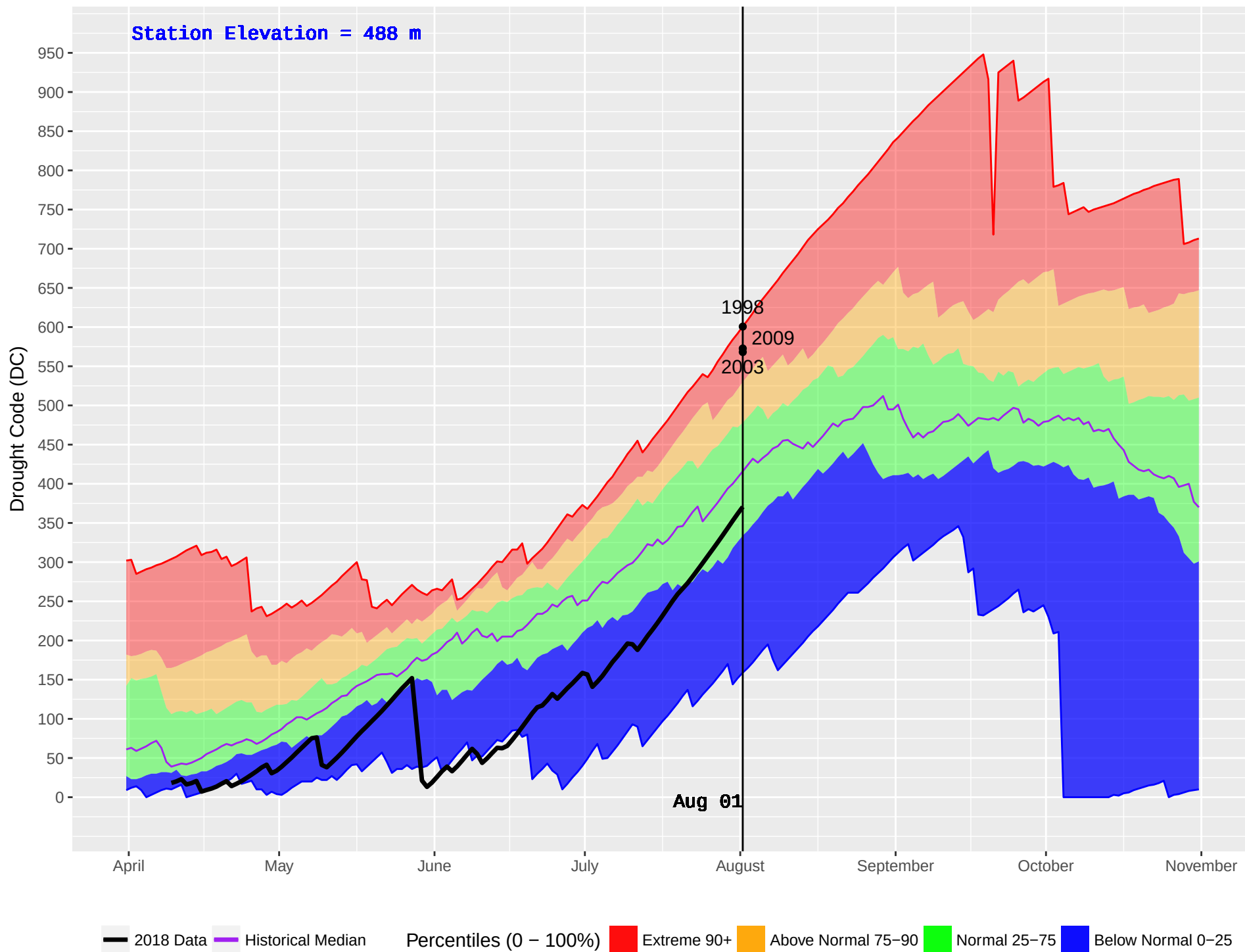
MABEL LAKE 2 (362) : Historical (1987–2016) and Current (2018) Daily Drought Code (DC)
